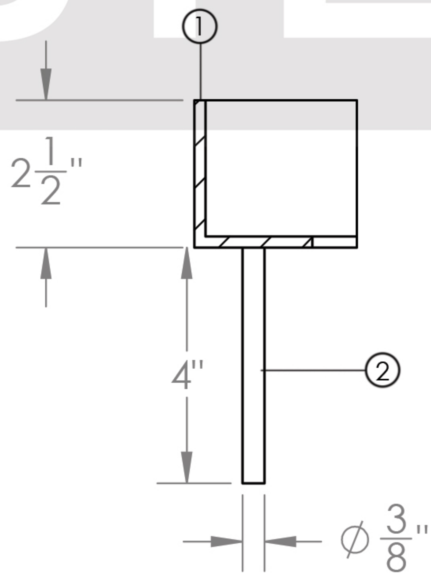
SECTION B-B
