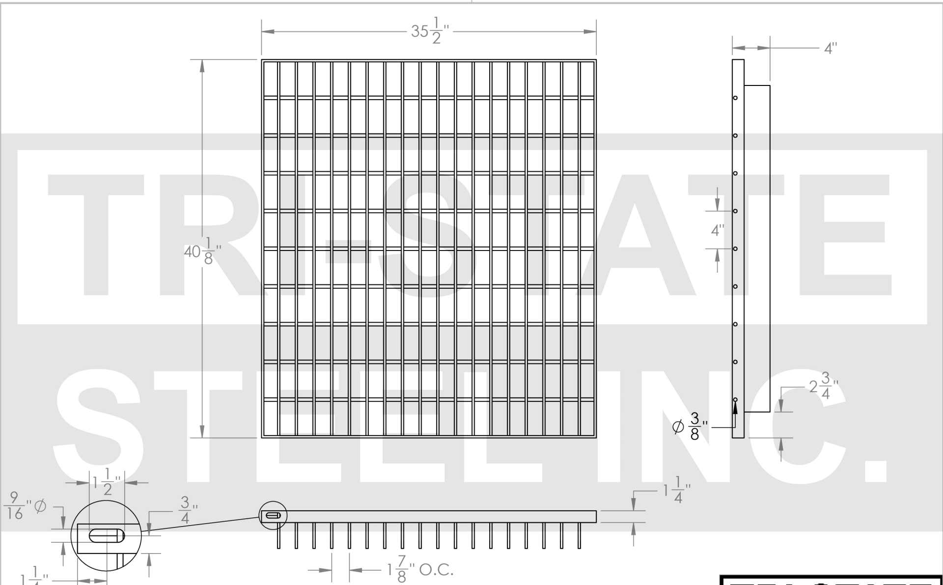
DETAIL A SCALE 1 : 4
